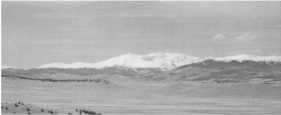
Altostratus clouds with cumulus on the right.
