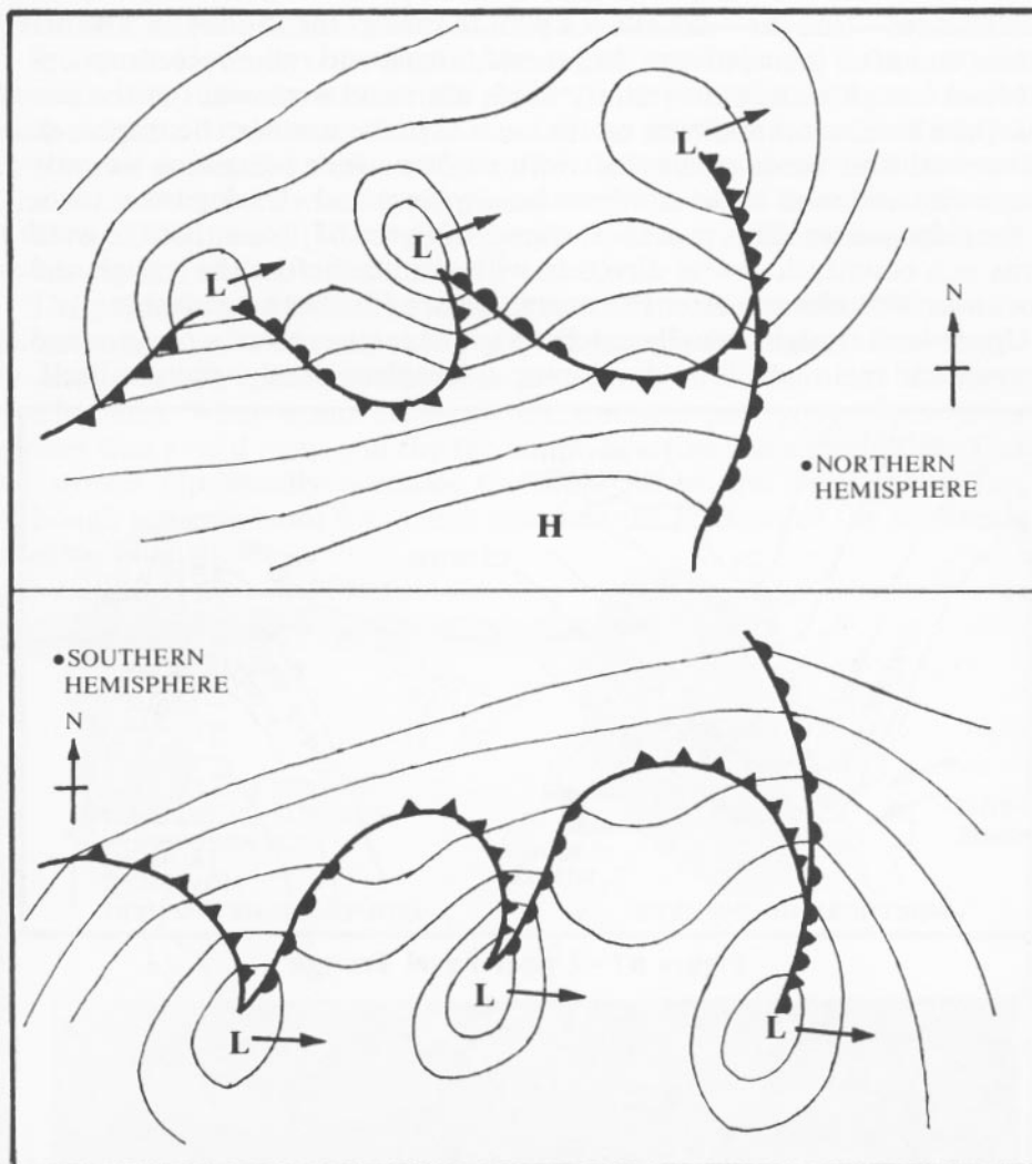
Figure 66 - Surface Waves
