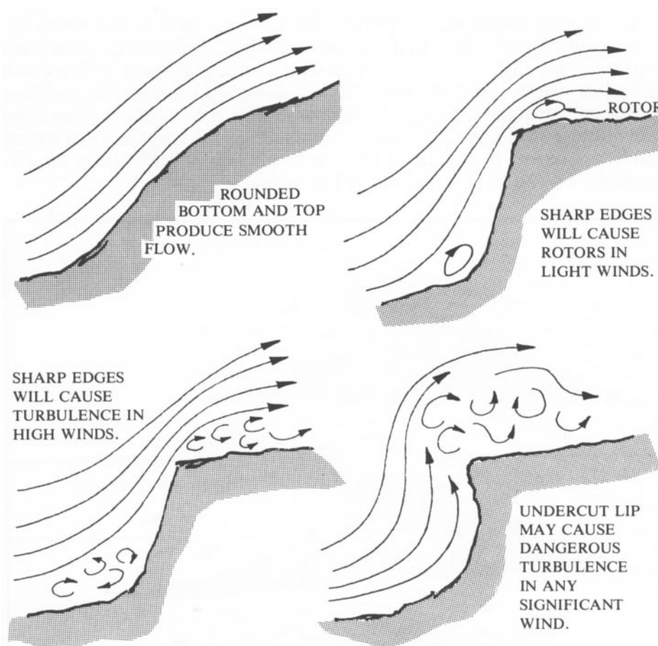
Figure 106 - Turbulence Near Hill Faces
