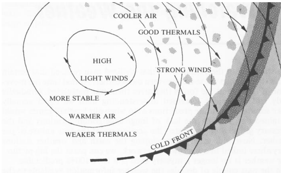
Figure 220 - Post-Frontal Conditions
