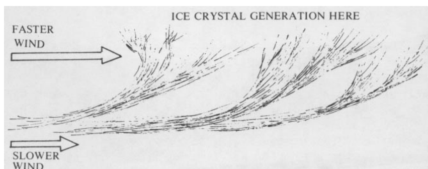
Figure 28 - Cirrus Clouds
