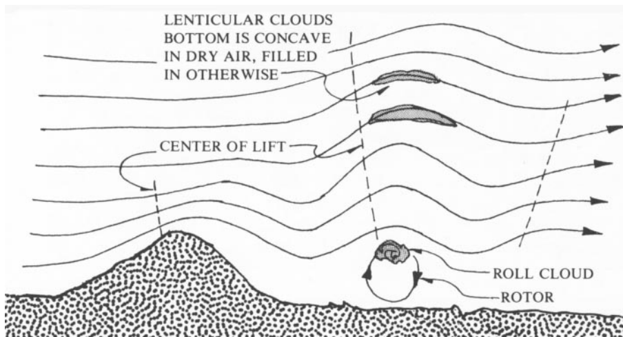
Figure 152 - Lenticular and Roll Clouds Associated with Waves
