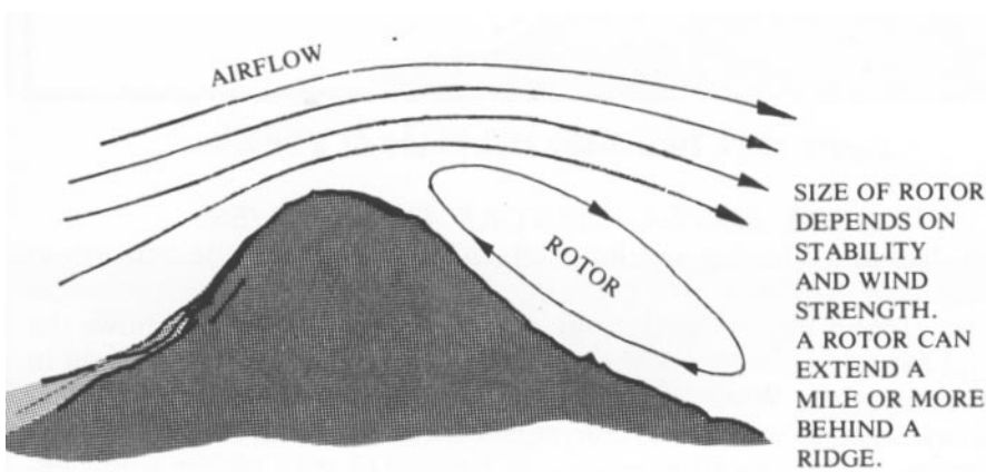
Figure 109 - Dangerous Lee Side Winds
