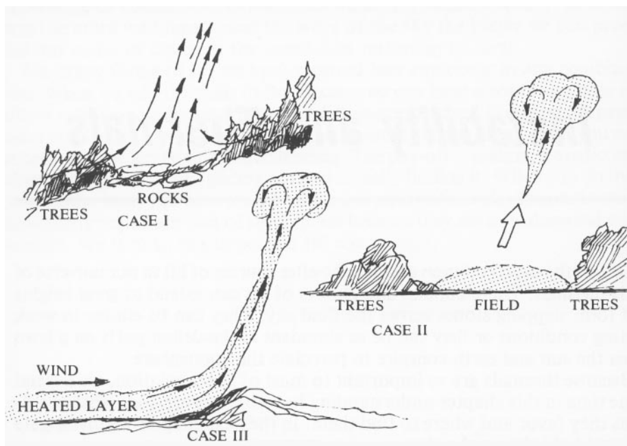
Figure 166 - Variations in Surface Conditions
