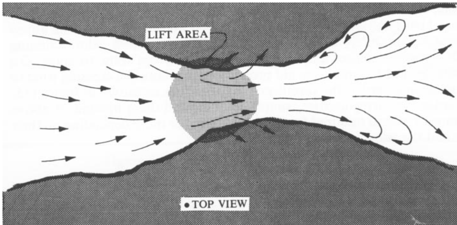
Figure 112 - Higher Winds in a Narrowing Channel
