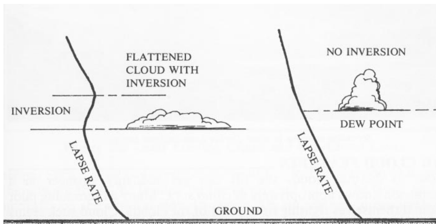
Figure 203 - Thermal Clouds With and Without an Inversion
