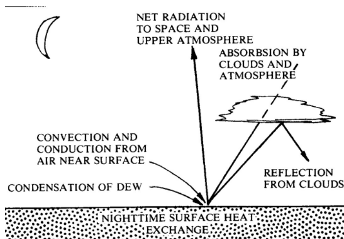
Figure 6 - Heat Radiation
